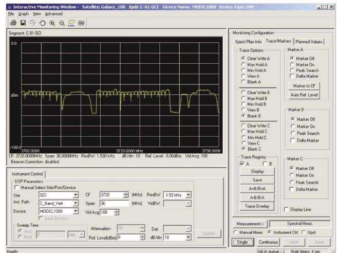
Figure 3 shows a spectrum analyzer image of the T1 SCPC traffic on one of GCI's transponders.
