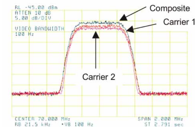
Figure 2. With DoubleTalk carrier-in-carrier.
