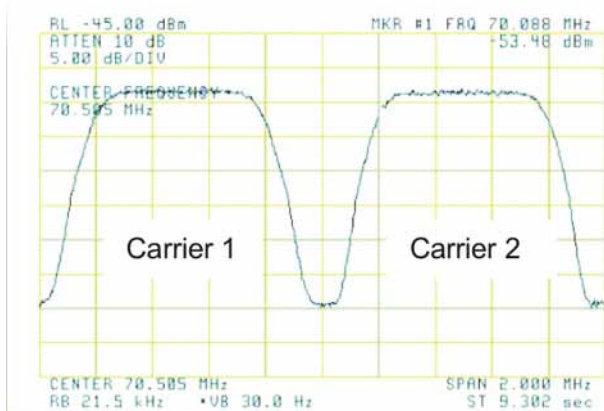
Figure 1. Without DoubleTalk carrier-in-carrier.
